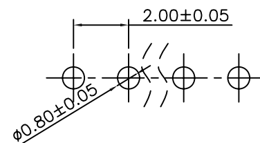
Recommended P.C.B Layout (Top Side)
