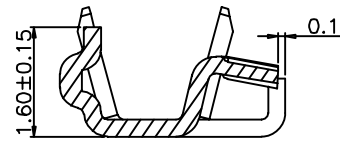
SEC:C-C
