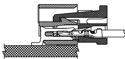
Assembly Layout
